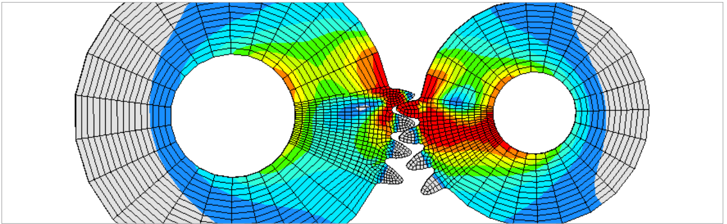
Von Mises stress plot of gears using a sliding contact
