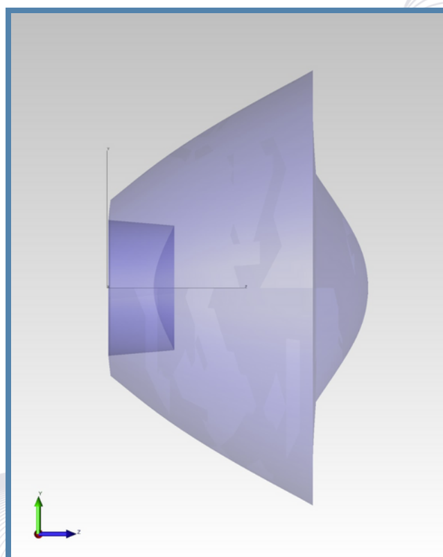
Figure 6a: Intensity plots for TIR hybrid lens with point source and ray file
