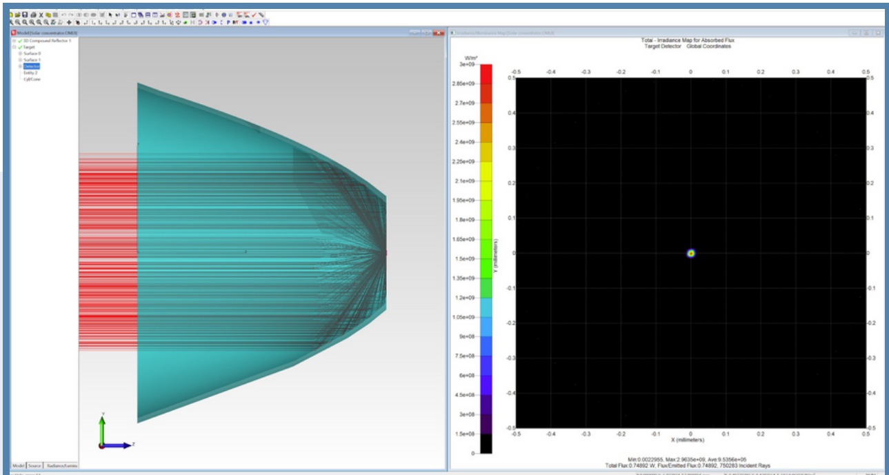
Figure 7: Irradiance plot for solar concentrator with parallel rays
