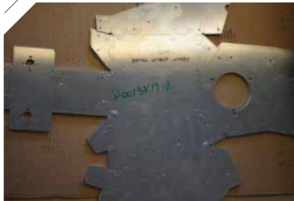
The Deep Orange 3 team worked hard to create folding pattern geometries as large as possible, the optimal way to fold them, and ways to nest parts to minimize material waste.
