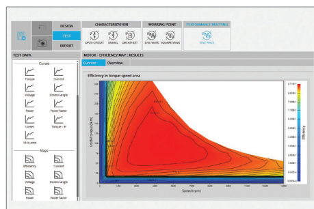
Efficiency map
