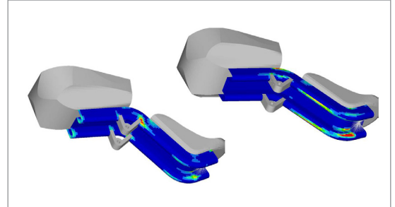
Composite chassis free-size optimization with Altair OptiStruct
