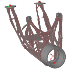
Inspire Optimization of steering column
