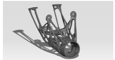
Rendering of new steering column after refinement with PolyNURBS
