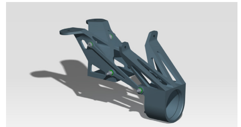
Original steering column assembly
