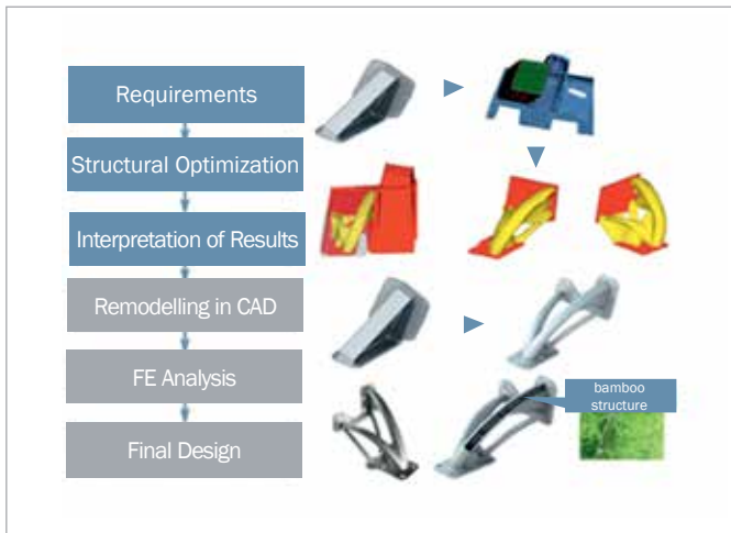
Newly developed process chain for the design and optimization of additively manufactured components
