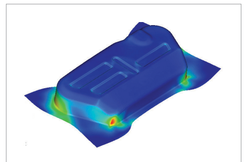
Plastic Strain
