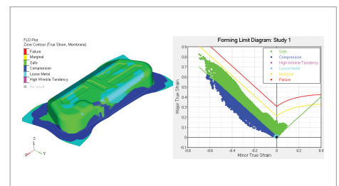
FLD Plot
