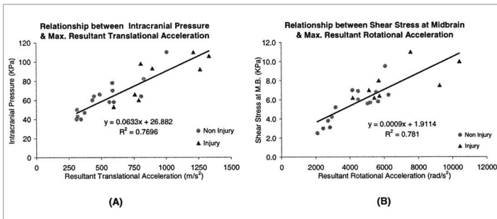
Fig. 3 Relationship Between Intracranial Pressure and the Maximum Translational Acceleration (A) and Between Shear Stress the Mid-Brain and Maximum Rotational Acceleration of the Head (B)
