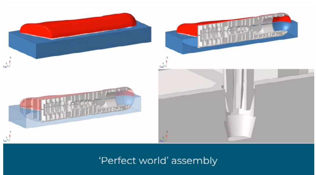
Structural analysis of a medical auto-injector during part assembly.
