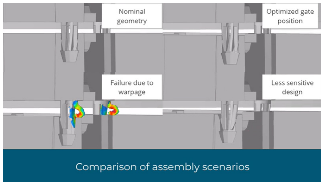
Structural analysis of a medical auto-injector during part assembly.
