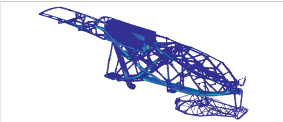
The optimization result represents the ideal geometry and is very close to the final structure of the additively manufactured part
