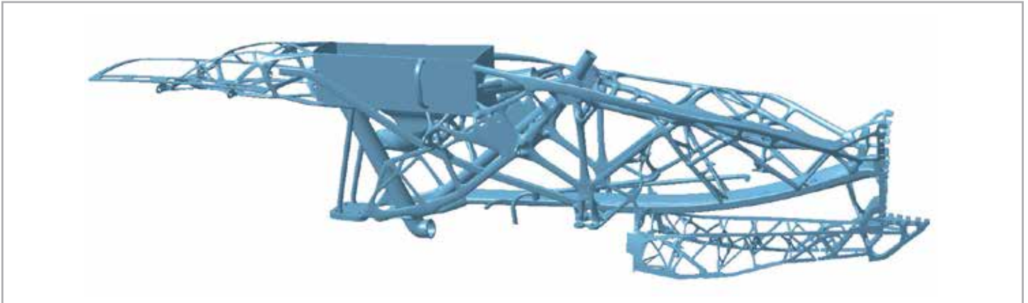
Final refined geometry of the engine pylon based on the optimization results and ready for the additive layer manufacturing. Compared to the traditional development and manufacturing methods, a weight saving of about 20 percent can be achieved.
