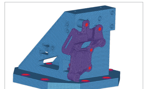
Fixture with Compressor Mounting Bracket
