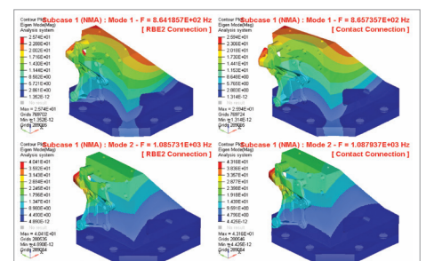
Mode Shape of Compressor Mounting Bracket with Fixture
