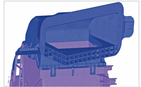
Fresh Air Duct (FAD) in HVAC Assembly
