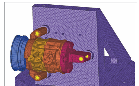
Fixture with Compressor Assembly
