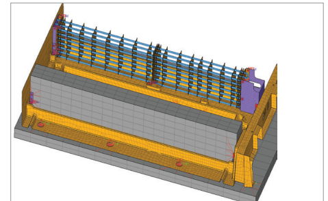
Evaporator Assembly (midsection with variable thickness of baseplate)
