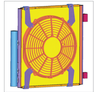
Condenser Assembly with Shroud Fan Assembly
